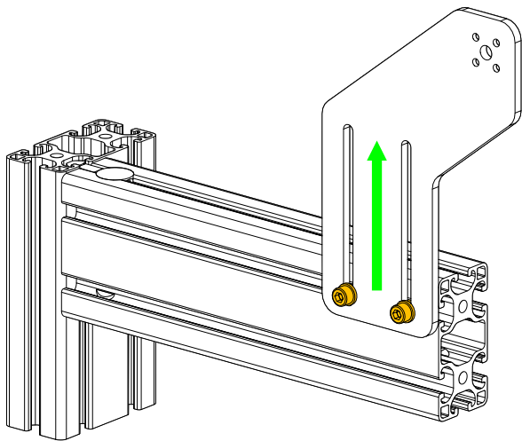
Alternative mounting allows for higher collective positions.
