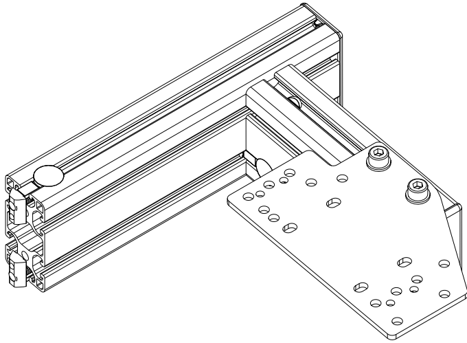
horizontal handbrake assembly
