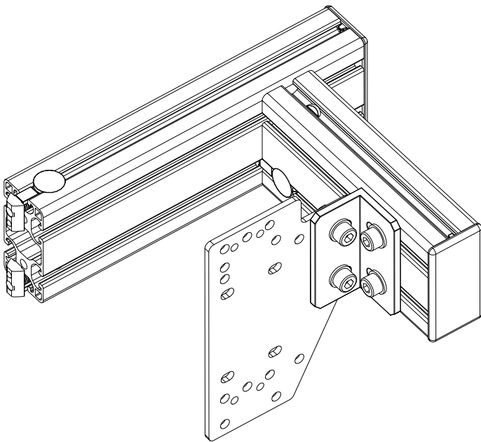
vertical handbrake assembly
